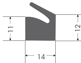
KC - 0051 KAPAK CONTASI COVER GASKET
