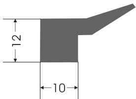
KC - 0053 KAPAK CONTASI COVER GASKET
