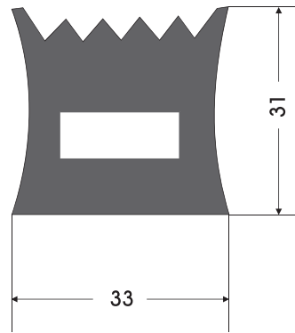
DT - 1 DIŞ TAMBUR LASTİĞİ OUTSIDE MAINWINCH RUBBER
