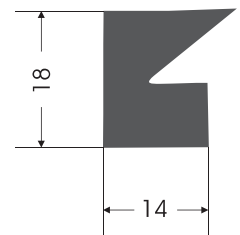
KC - 0024 KAPAK CONTASI COVER GASKET
