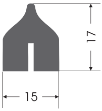
KC - 0041 KAPAK CONTASI COVER GASKET
