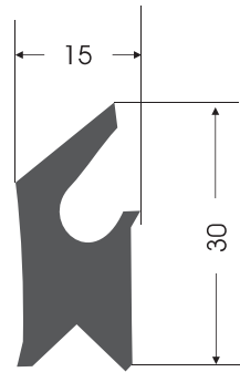
KC - 0003 KAPAK CONTASI COVER GASKET
