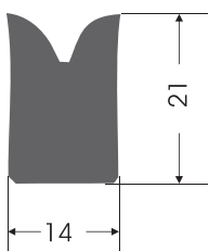
KC - 0009 KAPAK CONTASI COVER GASKET
