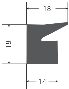
KC - 0025 KAPAK CONTASI COVER GASKET
