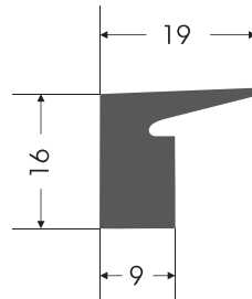
KC - 0047 KAPAK CONTASI COVER GASKET
