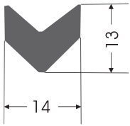
KC - 0013 KAPAK CONTASI COVER GASKET
