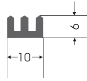
KC - 0043 KAPAK CONTASI COVER GASKET
