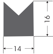
KC - 0014 KAPAK CONTASI COVER GASKET
