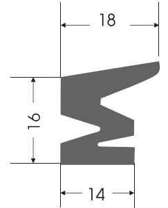
SC - 0001 SENKRON CONTASI COVER GASKET
