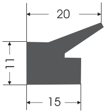
KC - 0025 KAPAK CONTASI COVER GASKET
