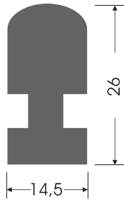
ÇB - 0001 ÇİLE BOYAMA KAPAK CONTASI SKEIN DYING COVER GASKET
