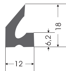
KC - 0060 KAPAK CONTASI COVER GASKET
