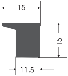
KC - 0037 KAPAK CONTASI COVER GASKET
