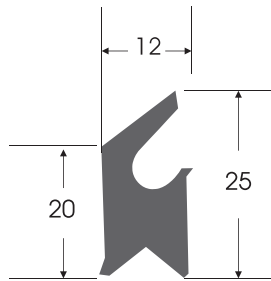
KC - 0002 KAPAK CONTASI COVER GASKET
