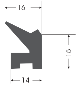
KC - 0040 KAPAK CONTASI COVER GASKET
