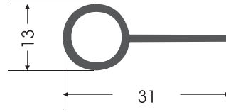
PP - 0015 P PROFİL P PROFILE
