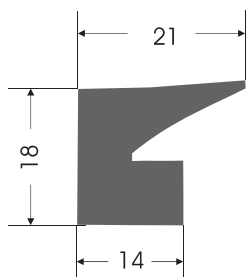
KC - 0026 KAPAK CONTASI COVER GASKET
