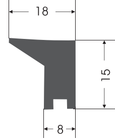
KC - 0039 KAPAK CONTASI COVER GASKET
