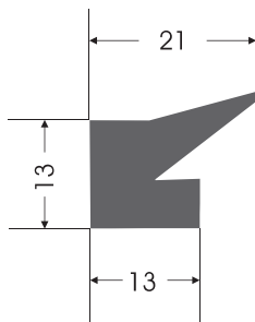
KC - 0022 KAPAK CONTASI COVER GASKET
