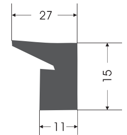
KC - 0028 KAPAK CONTASI COVER GASKET
