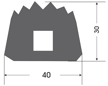
DT - 2 DIŞ TAMBUR LASTİĞİ OUTSIDE MAINWINCH RUBBER
