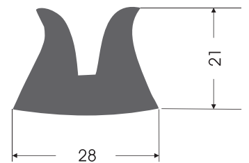
KC - 0012 KAPAK CONTASI COVER GASKET
