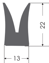
KC - 0010 KAPAK CONTASI COVER GASKET
