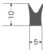
KC - 0006 KAPAK CONTASI COVER GASKET
