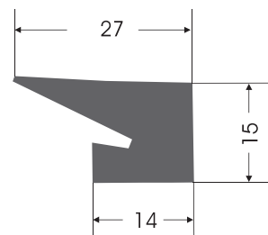
KC - 0035 KAPAK CONTASI COVER GASKET
