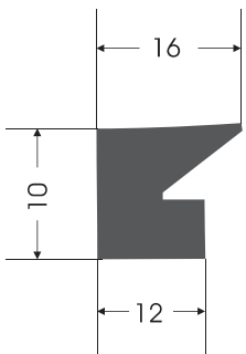
KC - 0021 KAPAK CONTASI COVER GASKET
