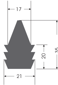
KC 0063 KAPAK CONTASI COVER GASKET
