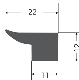
KC - 0052 KAPAK CONTASI COVER GASKET
