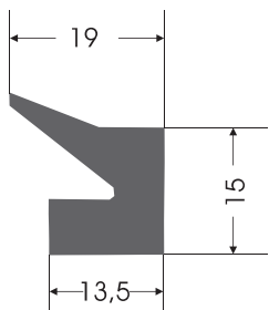
KC - 0029 KAPAK CONTASI COVER GASKET
