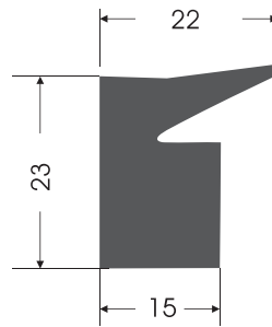
KC - 0027 KAPAK CONTASI COVER GASKET
