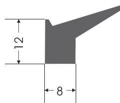
KC - 0055 KAPAK CONTASI COVER GASKET
