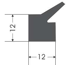
KC - 0048 KAPAK CONTASI COVER GASKET
