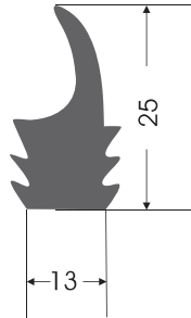
KC 0062 KAPAK CONTASI COVER GASKET
