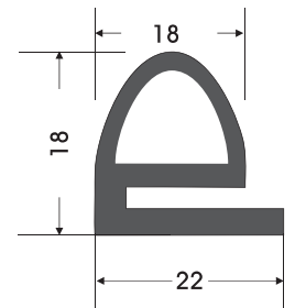
FC - 0003 FIRIN CONTASI OVEN GASKET
