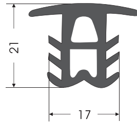
RC - 0006 RAMÖZ CONTASI MONFORTS STENTER GASKET
