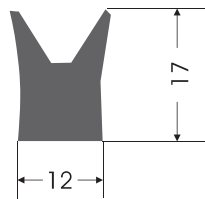
KC - 0007 KAPAK CONTASI COVER GASKET
