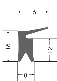
KC - 0059 KAPAK CONTASI COVER GASKET
