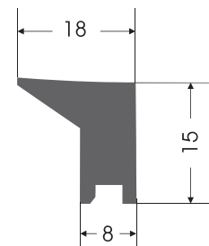
KC - 0056 KAPAK CONTASI COVER GASKET
