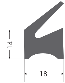
KC - 0061 KAPAK CONTASI COVER GASKET
