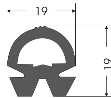
FC - 0002 FIRIN CONTASI OVEN GASKET
