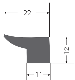
KC - 0030 KAPAK CONTASI COVER GASKET
