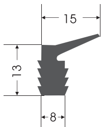
KC - 0049 KAPAK CONTASI COVER GASKET
