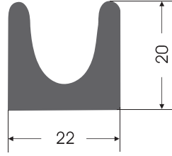
KC - 0042 KAPAK CONTASI COVER GASKET
