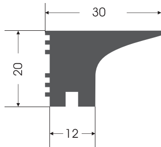
KC - 0046 KAPAK CONTASI COVER GASKET
