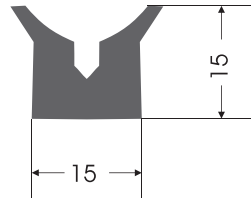
KC 0063 KAPAK CONTASI COVER GASKET
