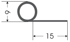
PP - 0013 P PROFİL P PROFILE
