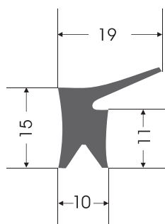
KC - 0054 KAPAK CONTASI COVER GASKET
