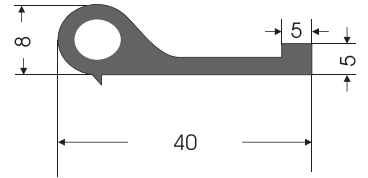
RC - 0007 RAMÖZ CONTASI MONFORTS STENTER GASKET
