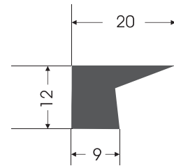
KC - 0027 KAPAK CONTASI COVER GASKET
