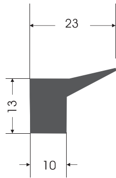
KC - 0030 KAPAK CONTASI COVER GASKET
