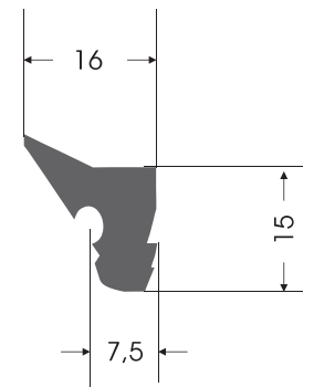
KC - 0004 KAPAK CONTASI COVER GASKET
