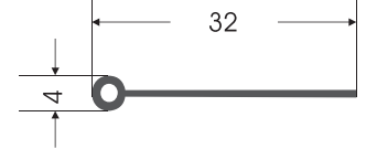
PP- 0016 P PROFİL P PROFILE
