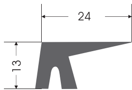
KC - 0050 KAPAK CONTASI COVER GASKET
