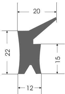
KC - 0057 KAPAK CONTASI COVER GASKET
