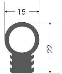
FC - 0001 FIRIN CONTASI OVEN GASKET
