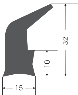
KC - 0001 KAPAK CONTASI COVER GASKET
